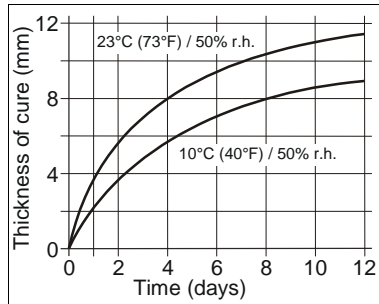
Diagram 1: Curing speed Sikaflex®-527 AT
